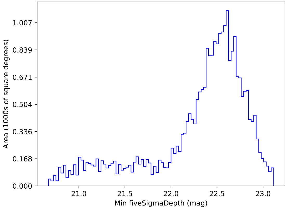
ddf_loaded_half_f14_v3.4_10yrs Yr 1 z band: Min fiveSigmaDepth
