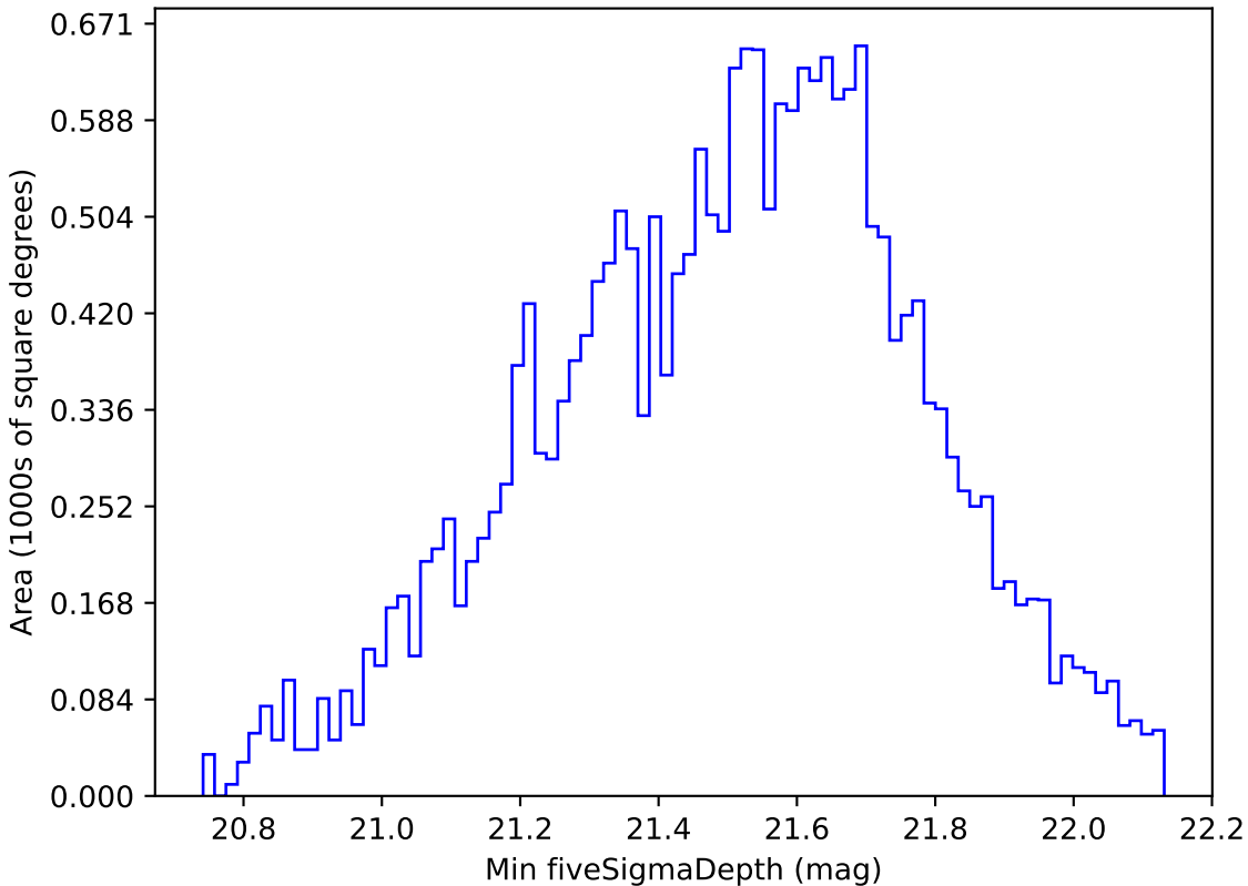
ddf_loaded_half_fl4_v3.4_10yrs Yr 1 y band: Min fiveSigmaDepth
