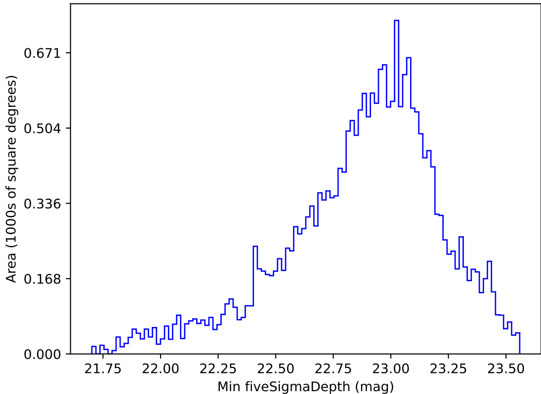
ddf_loaded_half_fl4_v3.4_10yrs Yr 1 u band: Min fiveSigmaDepth
