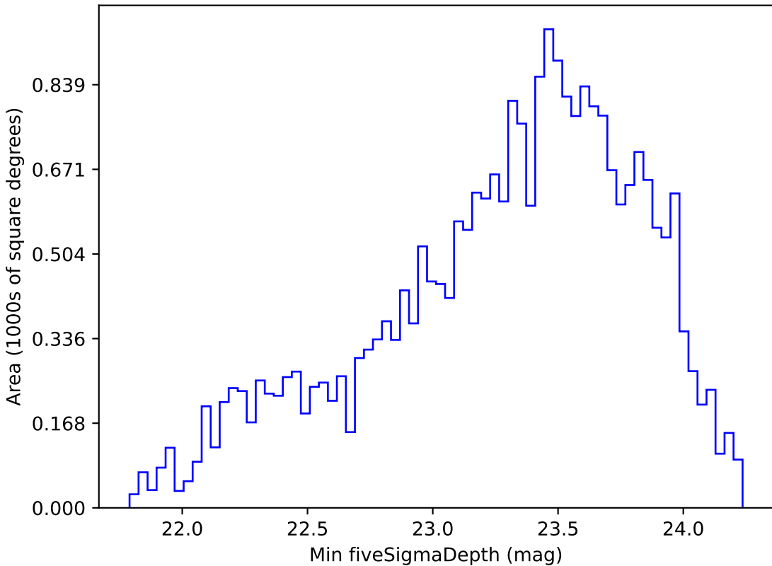
ddf_loaded_half_fl4_v3.4_10yrs Yr 1 r band: Min fiveSigmaDepth
