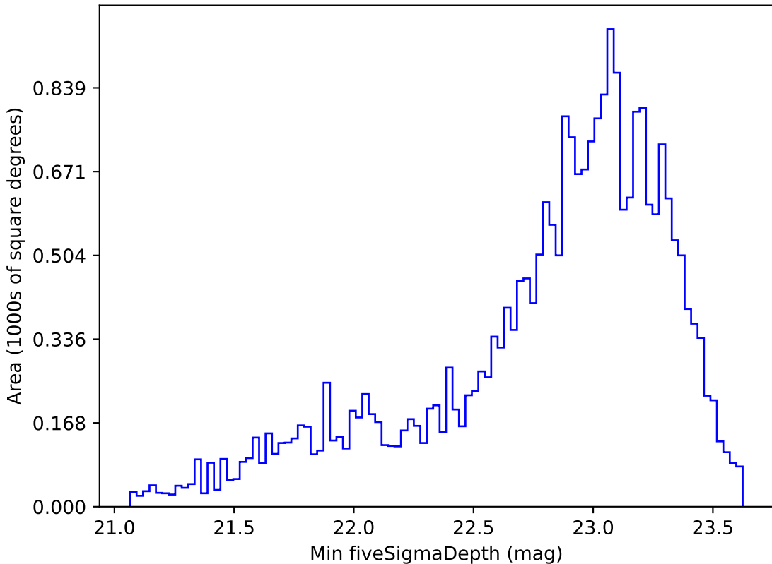
ddf_loaded_half_fl4_v3.4_10yrs Yr 1 i band: Min fiveSigmaDepth
