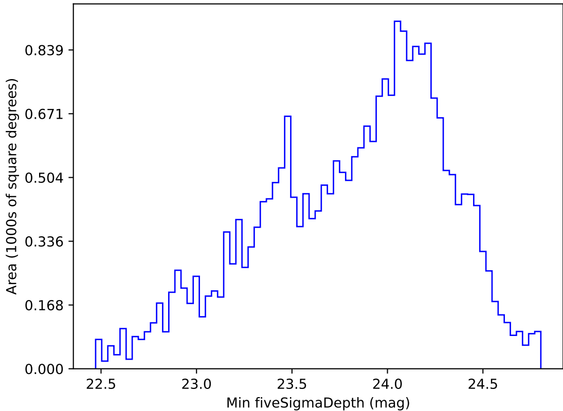
ddf_loaded_half_fl4_v3.4_10yrs Yr 1 g band: Min fiveSigmaDepth
