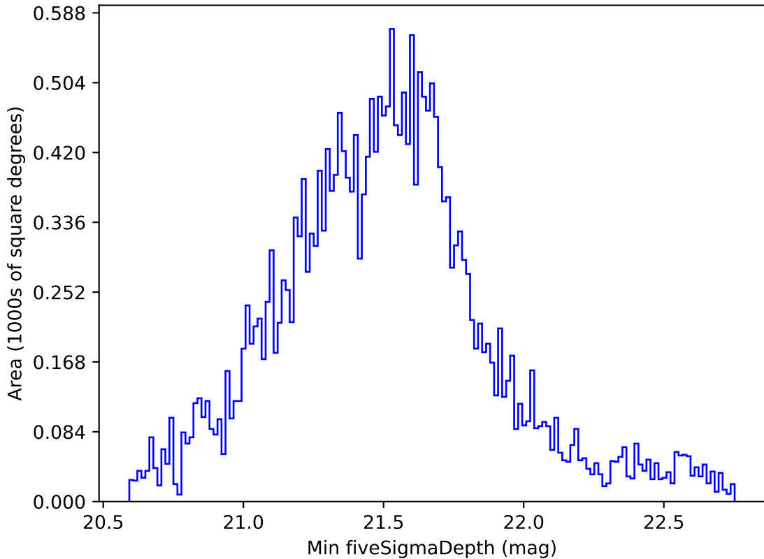
ddf_loaded_half_fl4_v3.4_10yrs Yr 1 all bands: Min fiveSigmaDepth
