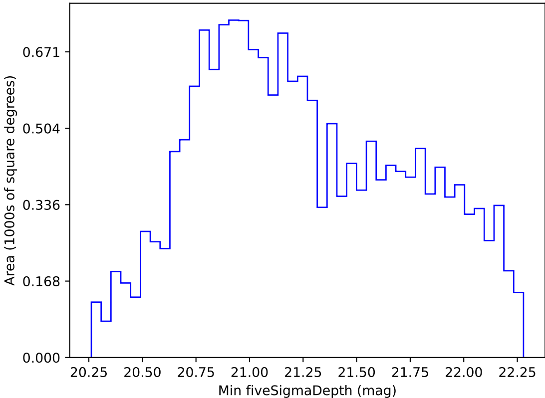
ddf_loaded_half_fl4_v3.4_10yrs WFD z band: Min fiveSigmaDepth
