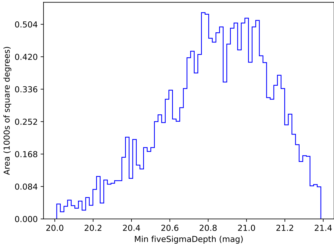
ddf_loaded_half_fl4_v3.4_10yrs WFD y band: Min fiveSigmaDepth
