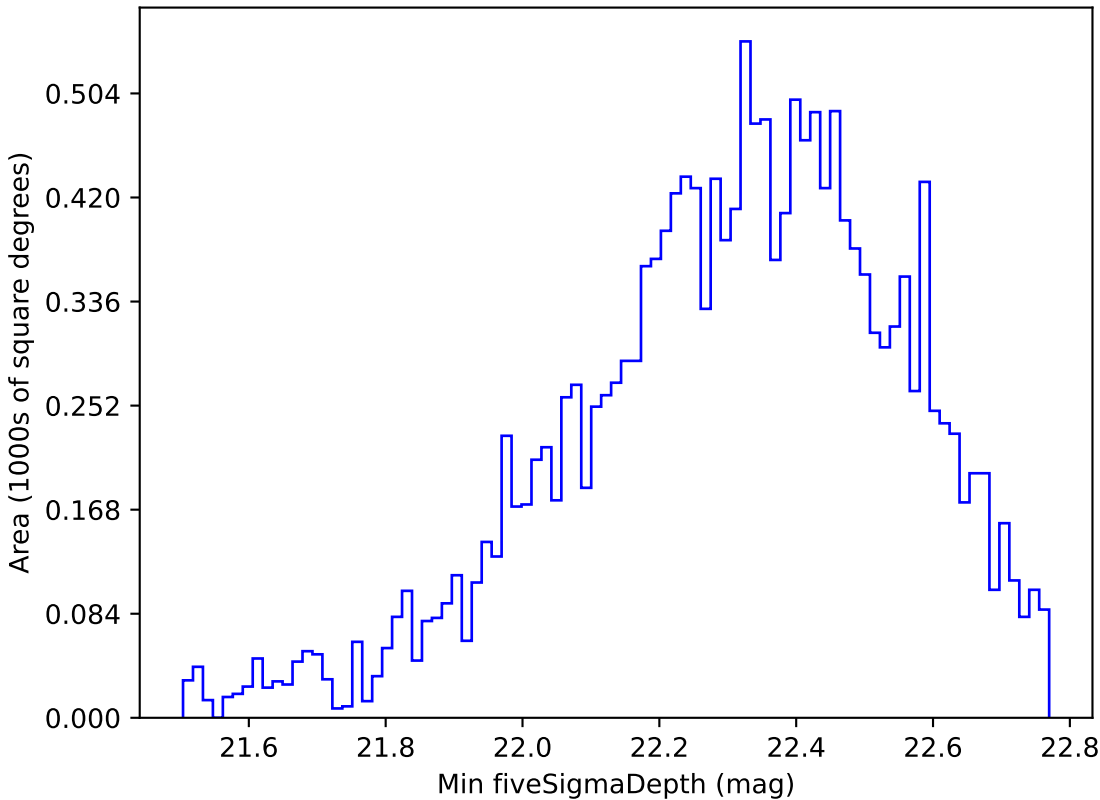
ddf_loaded_half_fl4_v3.4_10yrs WFD u band: Min fiveSigmaDepth
