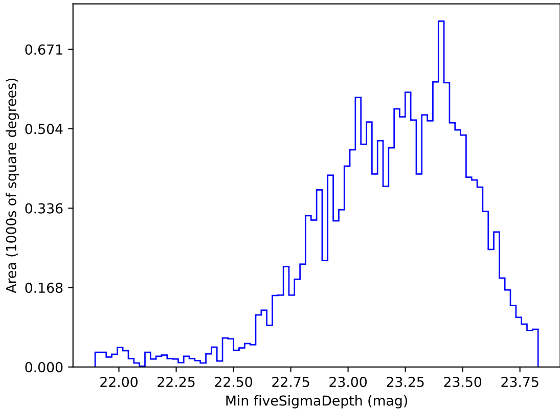
ddf_loaded_half_fl4_v3.4_10yrs WFD g band: Min fiveSigmaDepth
