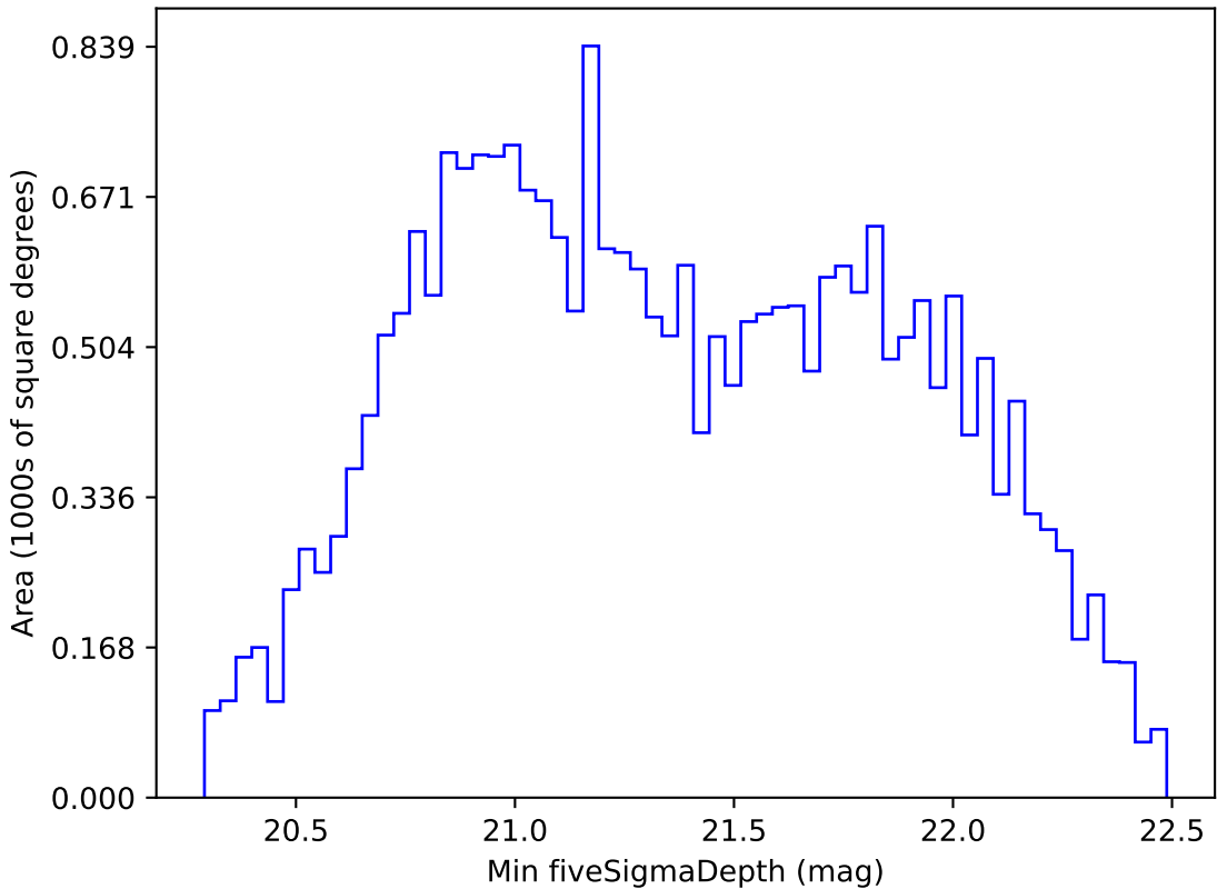
ddf_loaded_half_fl4_v3.4_10yrs All sky z band: Min fiveSigmaDepth
