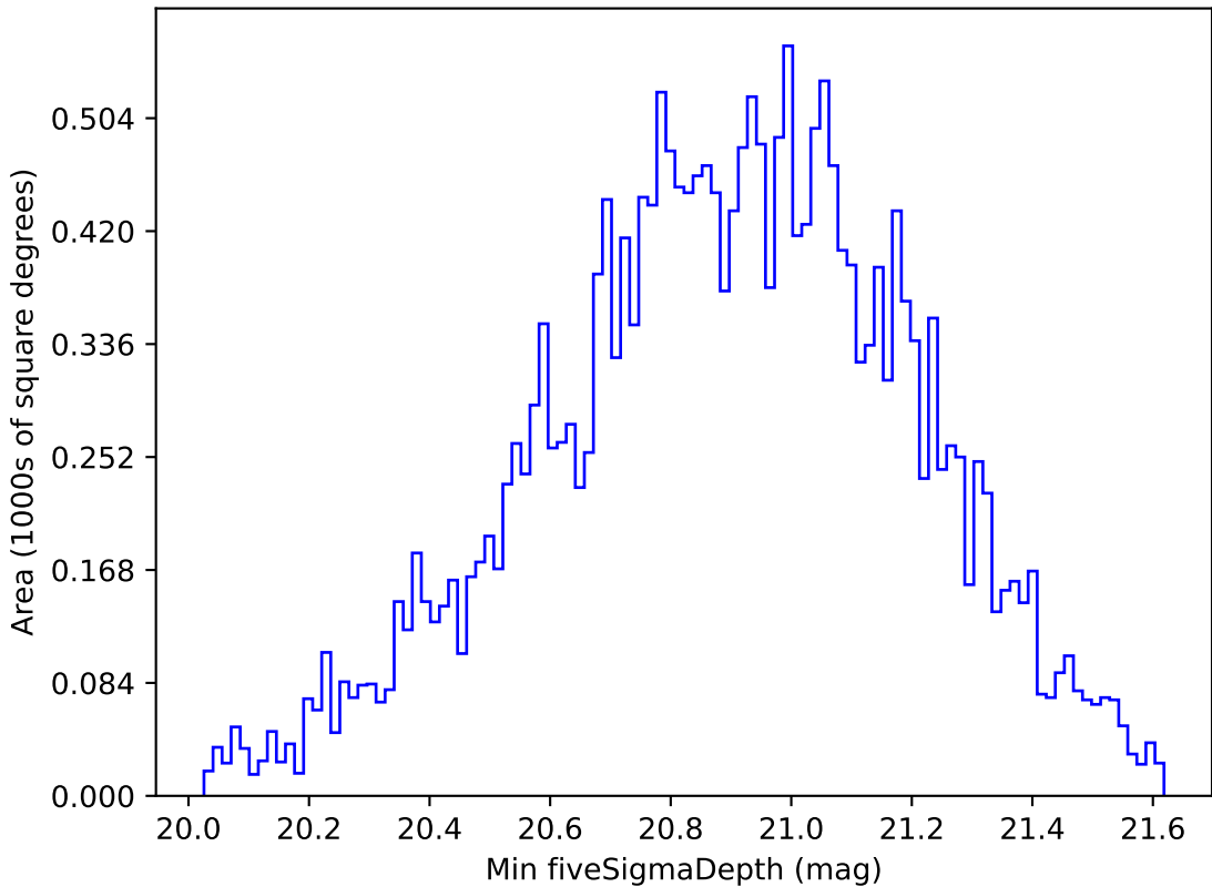
ddf_loaded_half_fl4_v3.4_10yrs All sky y band: Min fiveSigmaDepth
