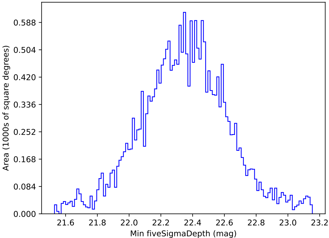
ddf_loaded_half_fl4_v3.4_10yrs All sky u band: Min fiveSigmaDepth
