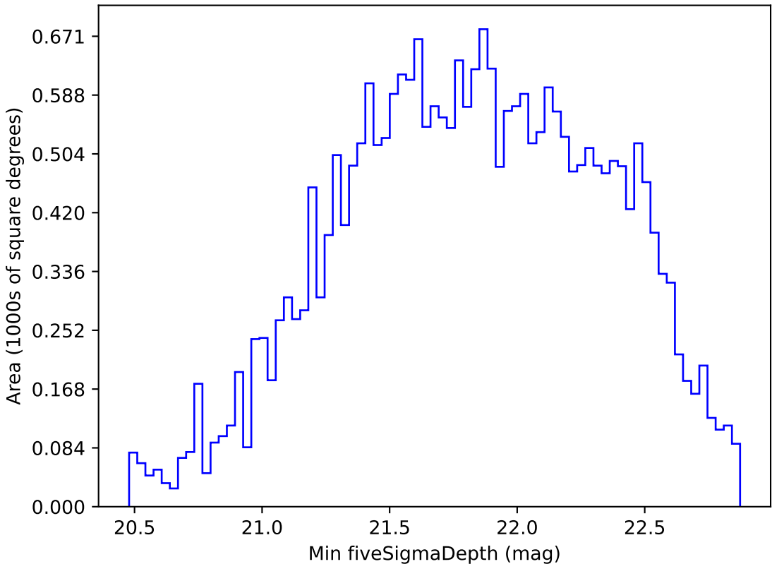
ddf_loaded_half_fl4_v3.4_10yrs All sky i band: Min fiveSigmaDepth
