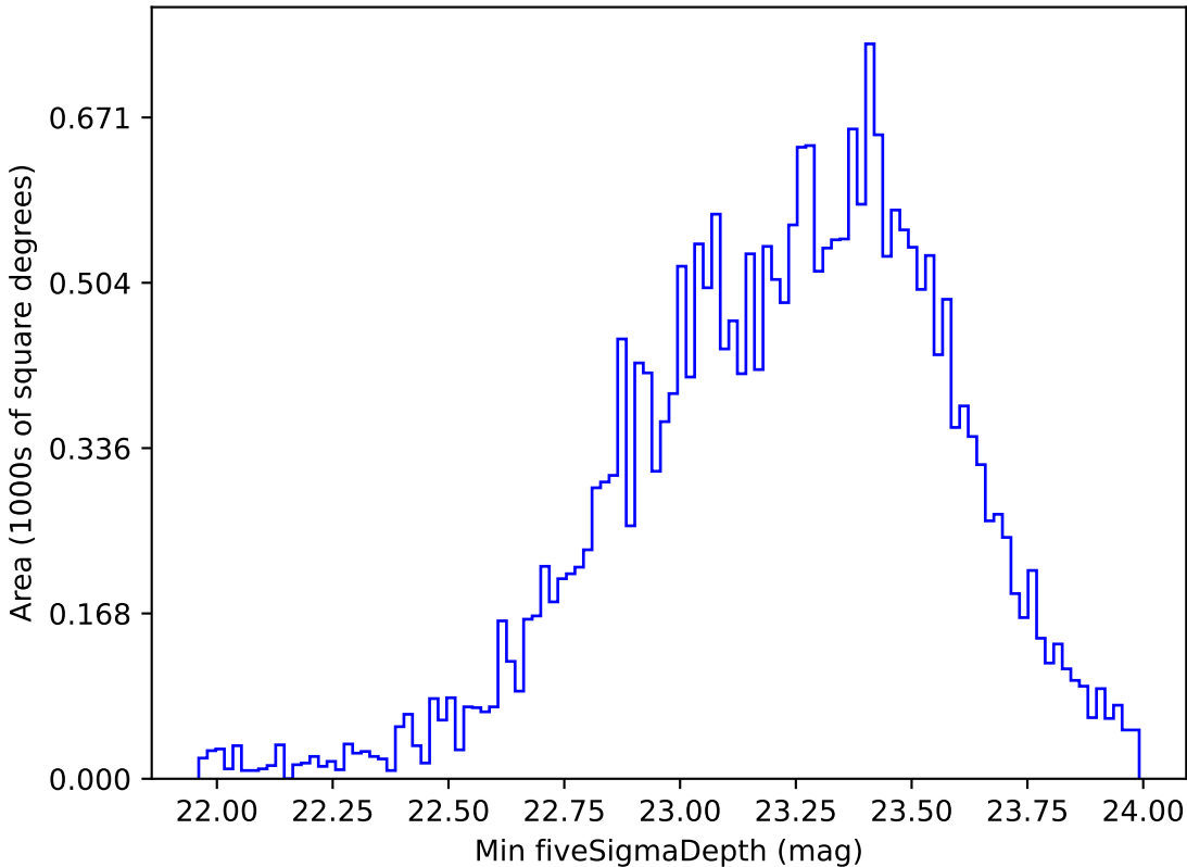
ddf_loaded_half_fl4_v3.4_10yrs All sky g band: Min fiveSigmaDepth
