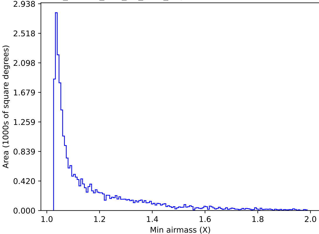
ddf_loaded_half_fl4_v3.4_10yrs Yr 1 z band: Min airmass
