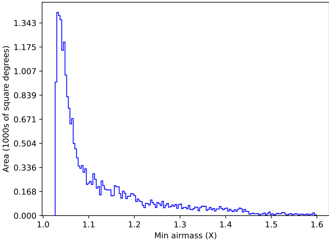
ddf_loaded_half_fl4_v3.4_10yrs Yr 1 y band: Min airmass
