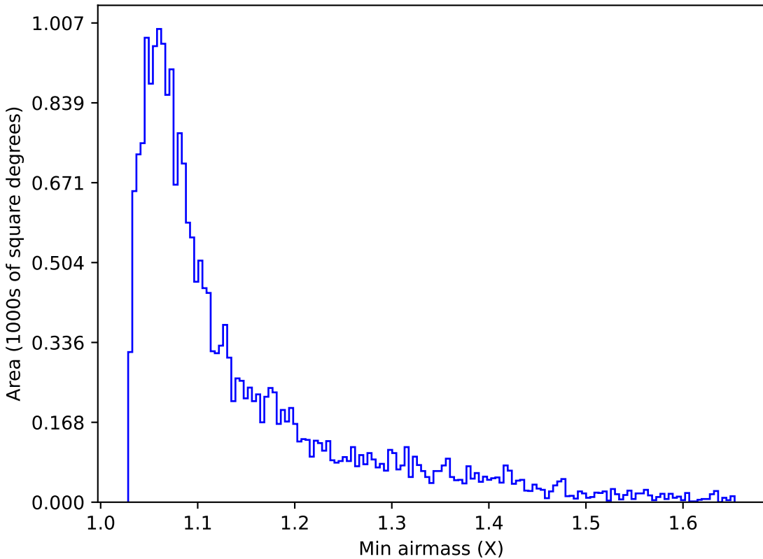
ddf_loaded_half_fl4_v3.4_10yrs Yr 1 u band: Min airmass
