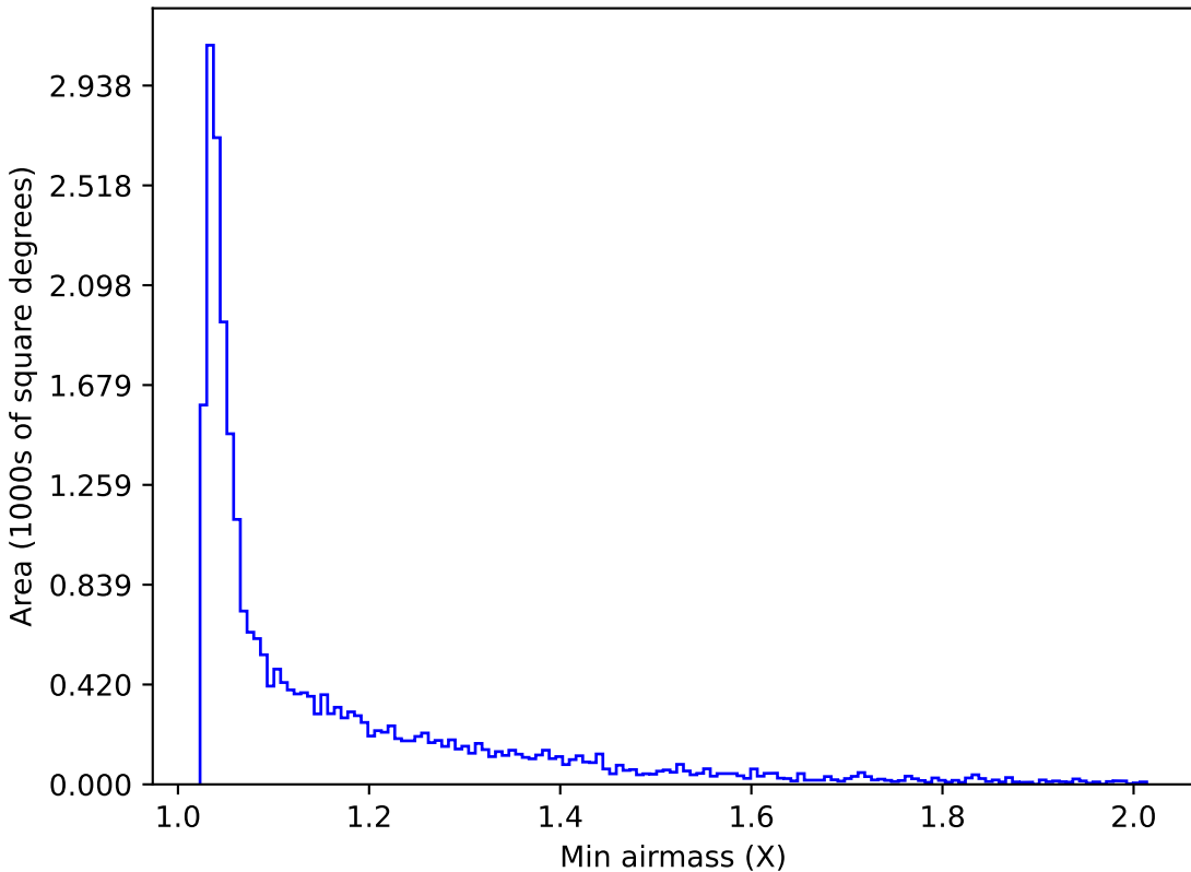
ddf_loaded_half_fl4_v3.4_10yrs Yr 1 r band: Min airmass
