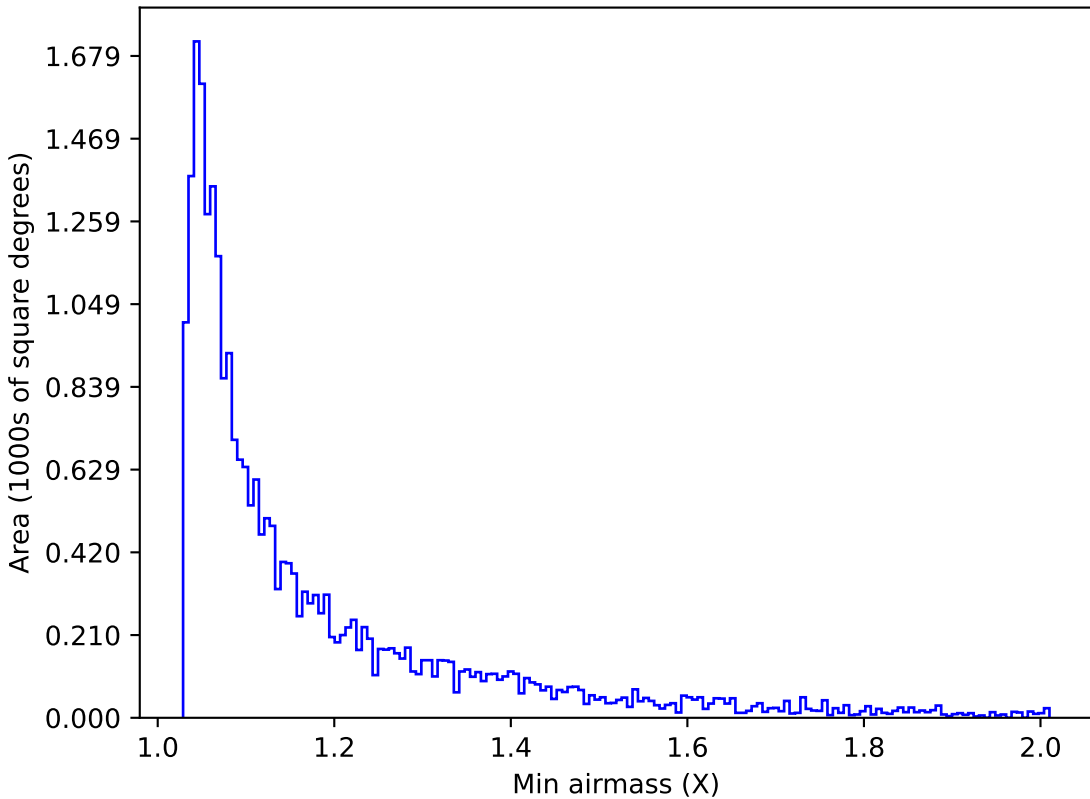
ddf_loaded_half_fl4_v3.4_10yrs Yr 1 g band: Min airmass
