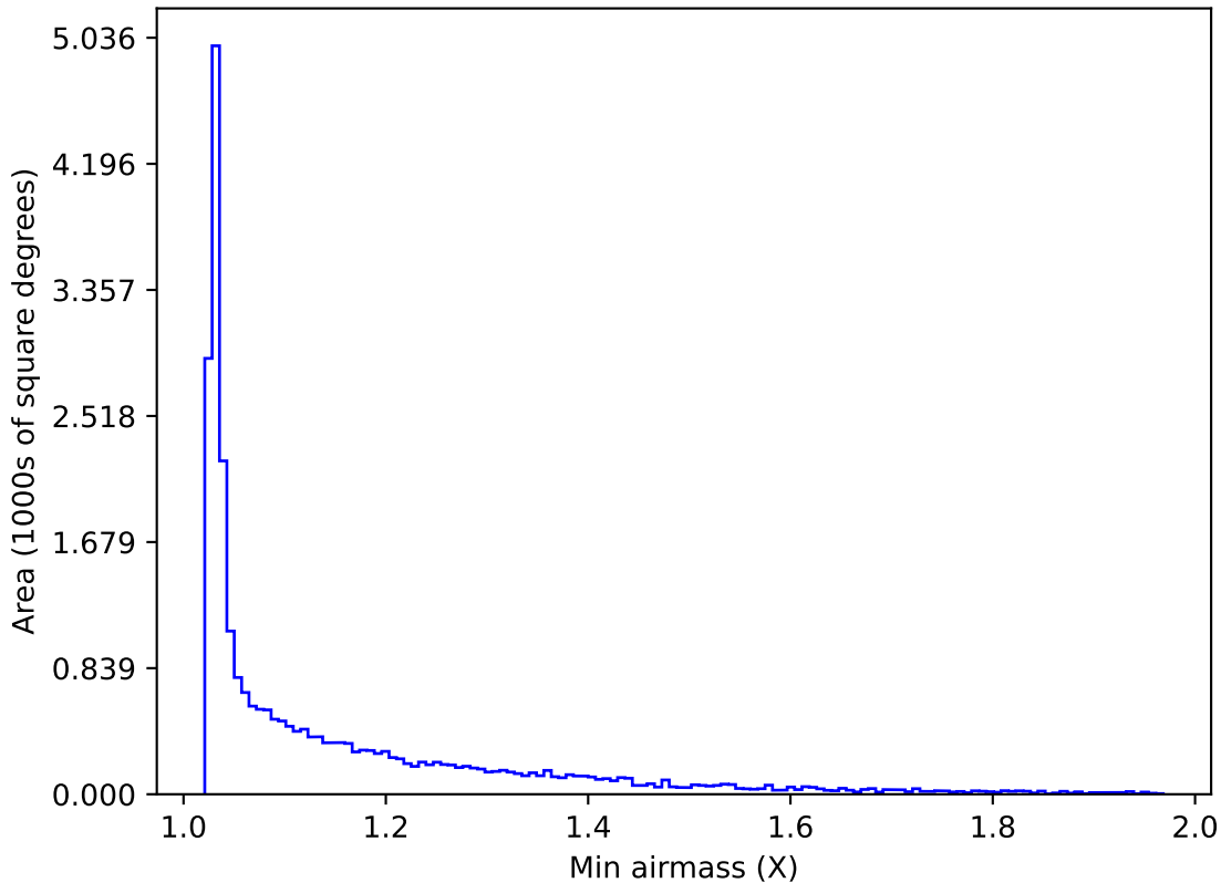
ddf_loaded_half_fl4_v3.4_10yrs Yr 1 all bands: Min airmass
