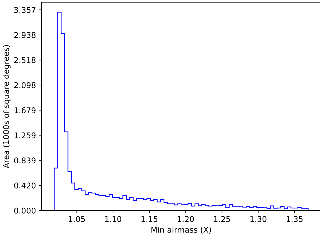
ddf_loaded_half_fl4_v3.4_10yrs WFD z band: Min airmass
