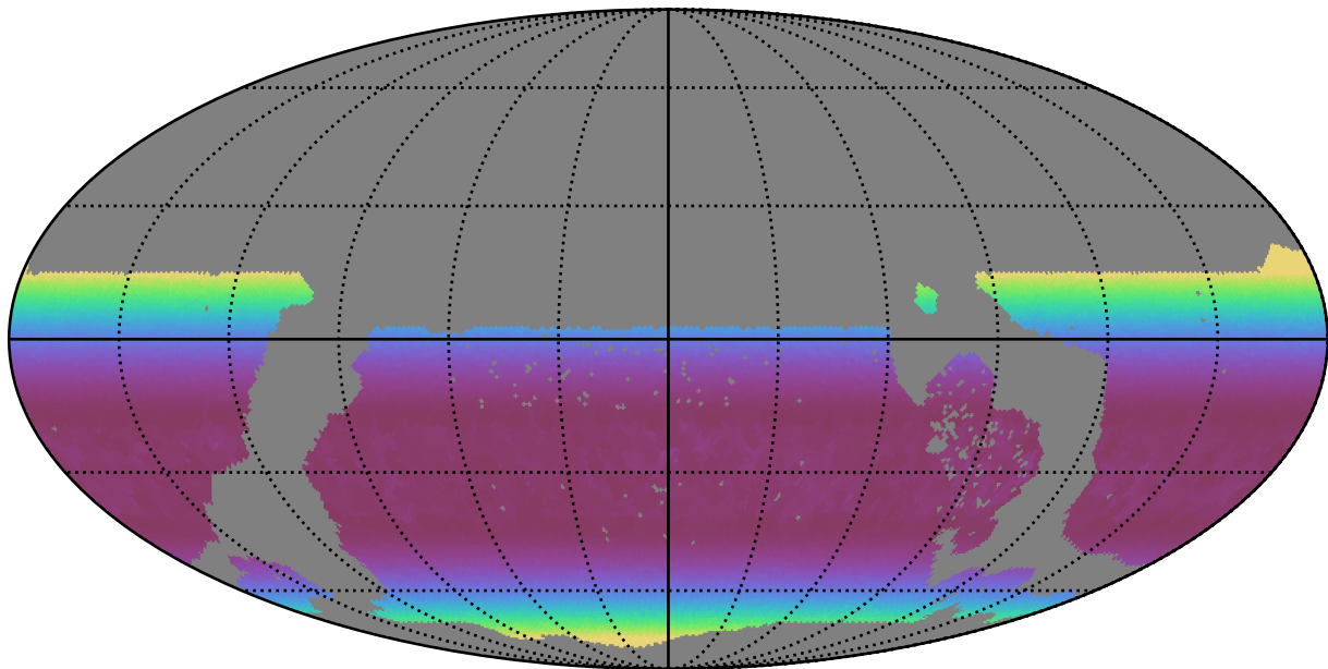
ddf_loaded_half_fl4_v3.4_10yrs WFD y band: Min airmass
