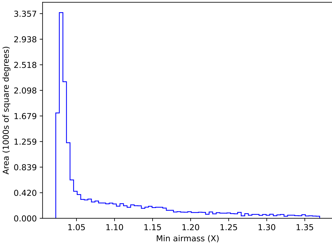
ddf_loaded_half_fl4_v3.4_10yrs WFD y band: Min airmass
