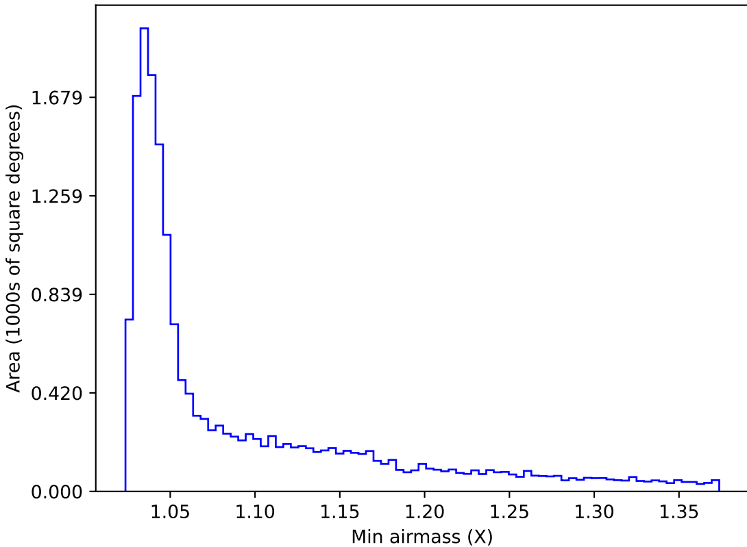
ddf_loaded_half_fl4_v3.4_10yrs WFD u band: Min airmass
