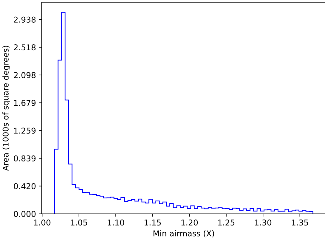
ddf_loaded_half_fl4_v3.4_10yrs WFD r band: Min airmass
