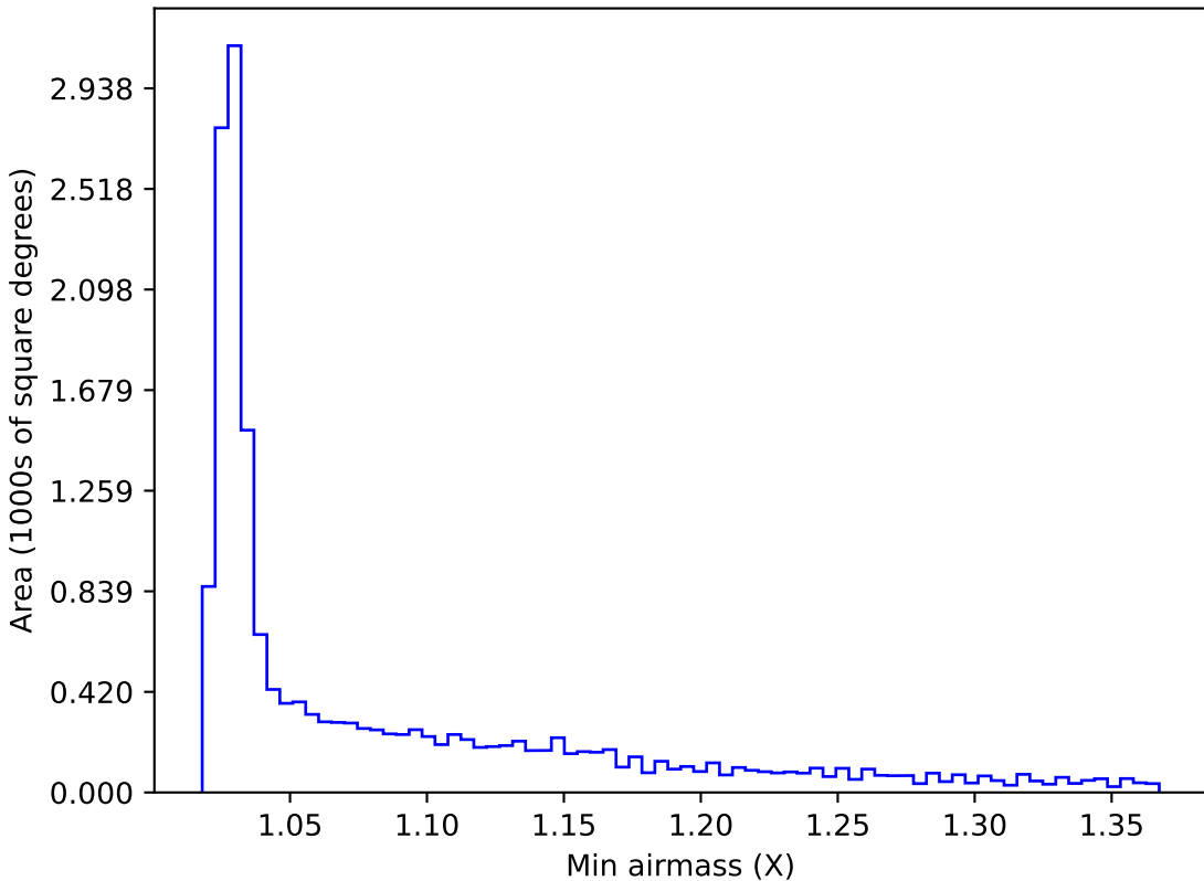
ddf_loaded_half_fl4_v3.4_10yrs WFD i band: Min airmass
