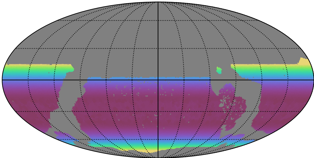
ddf_loaded_half_fl4_v3.4_10yrs WFD all bands: Min airmass
