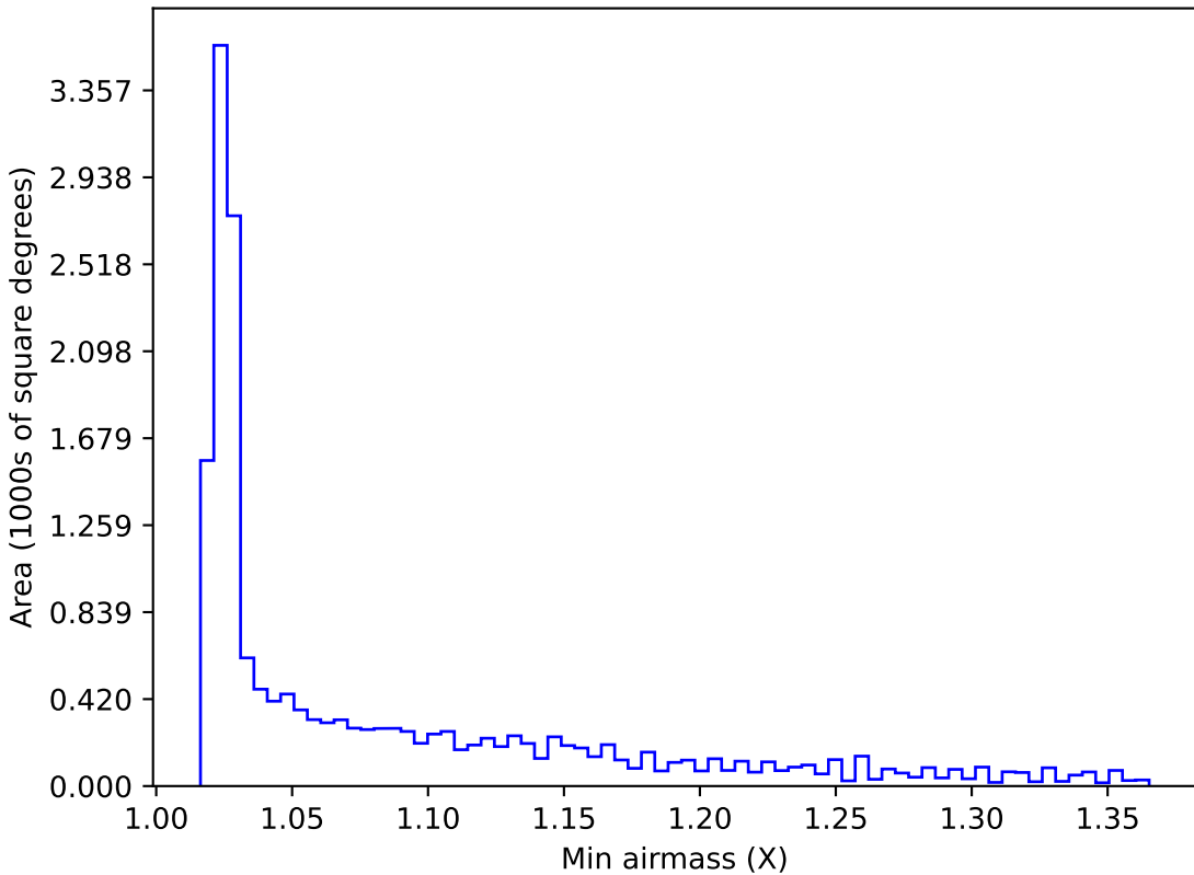
ddf_loaded_half_fl4_v3.4_10yrs WFD all bands: Min airmass
