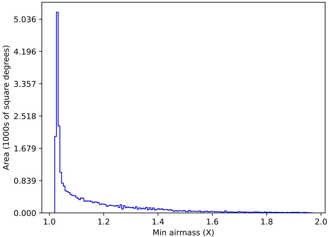
ddf_loaded_half_fl4_v3.4_10yrs All sky z band: Min airmass
