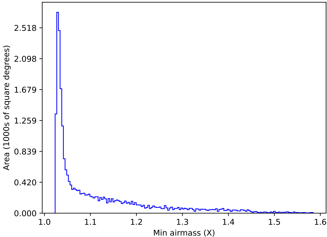
ddf_loaded_half_fl4_v3.4_10yrs All sky y band: Min airmass
