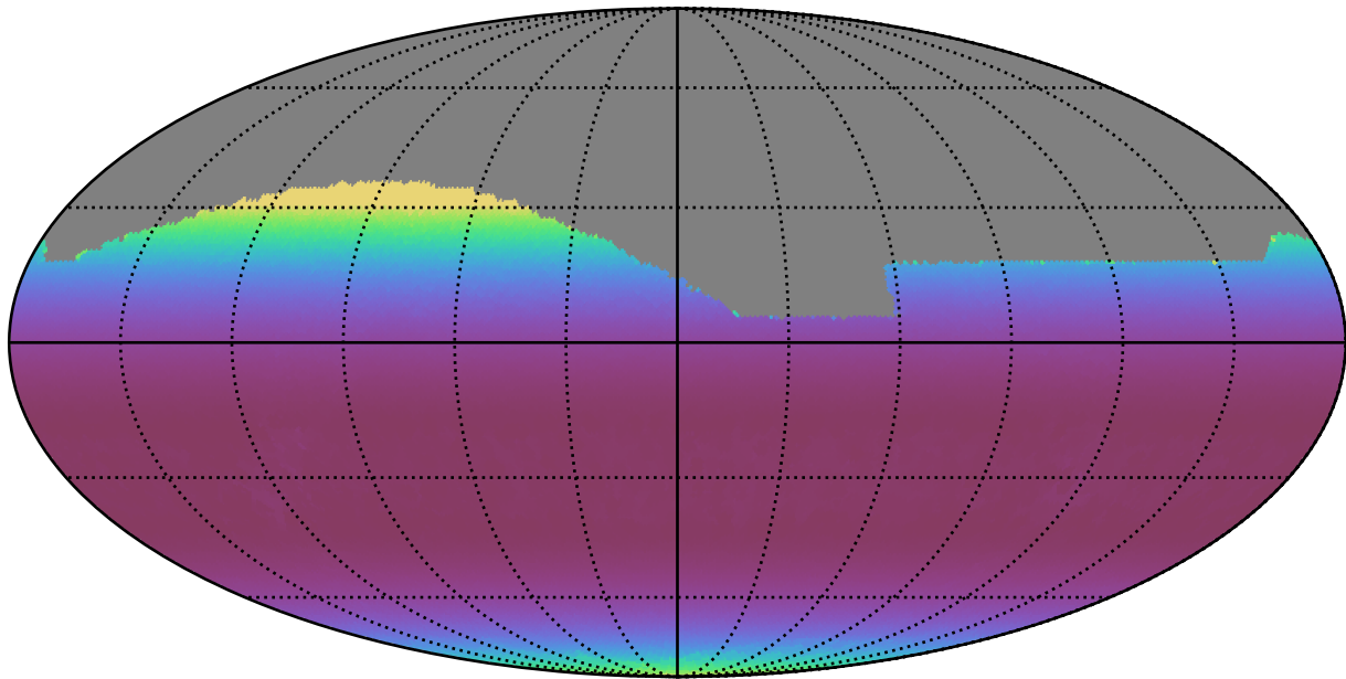
ddf_loaded_half_fl4_v3.4_10yrs All sky r band: Min airmass
