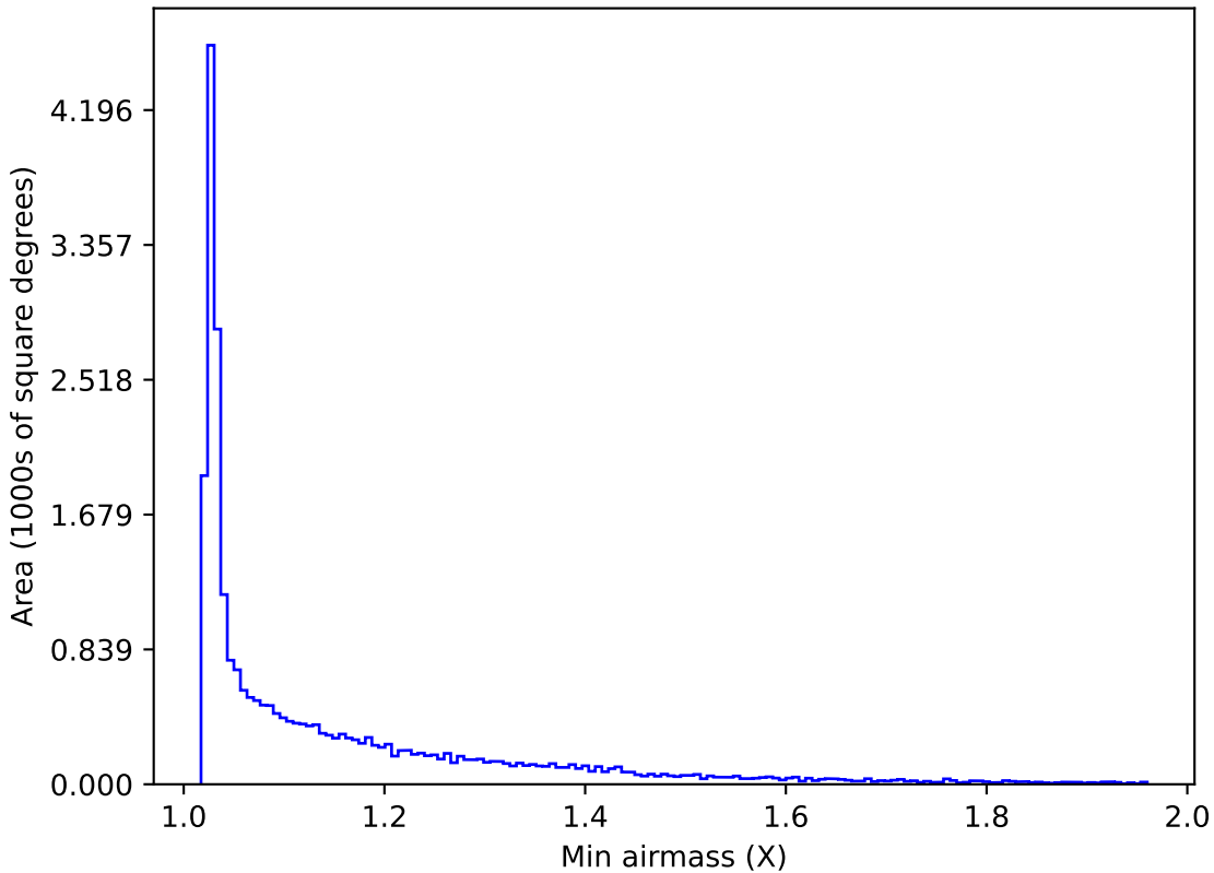
ddf_loaded_half_fl4_v3.4_10yrs All sky r band: Min airmass
