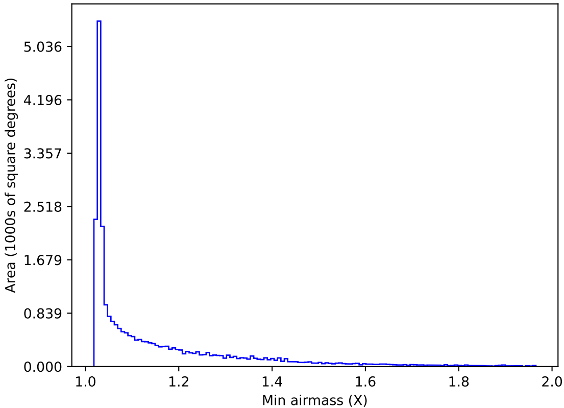
ddf_loaded_half_fl4_v3.4_10yrs All sky i band: Min airmass
