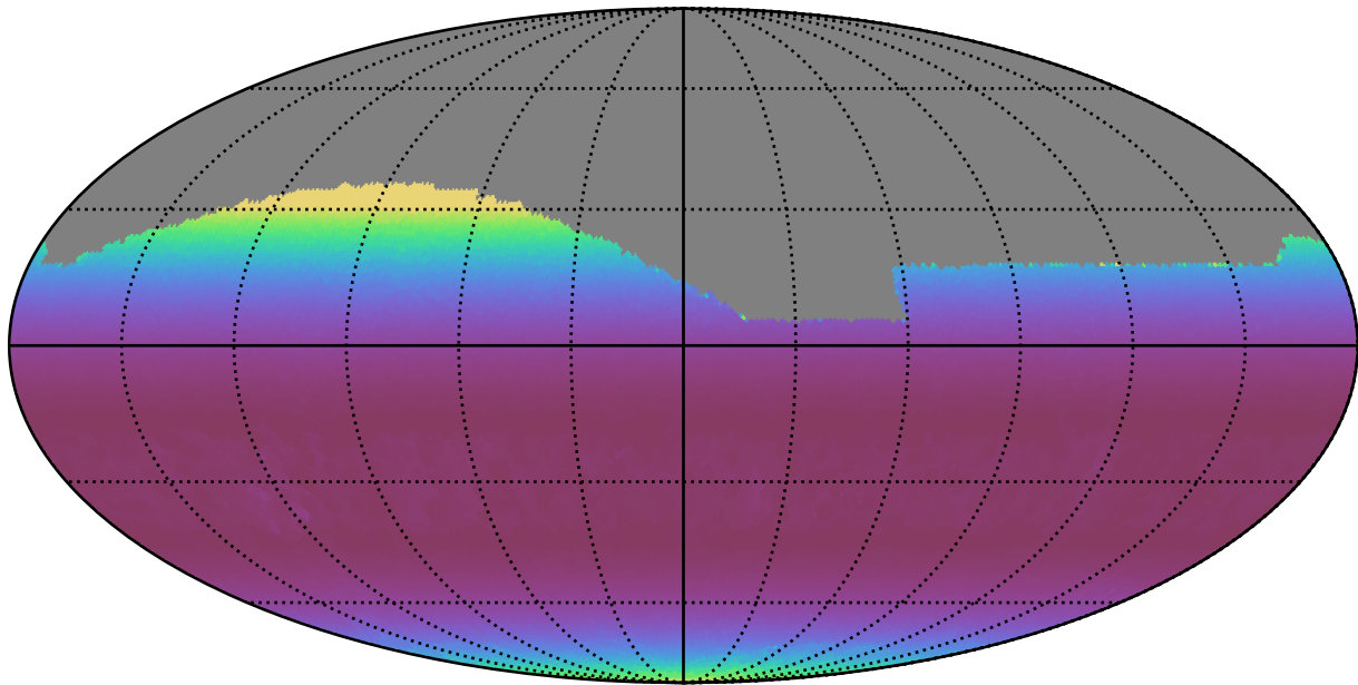
ddf_loaded_half_fl4_v3.4_10yrs All sky g band: Min airmass
