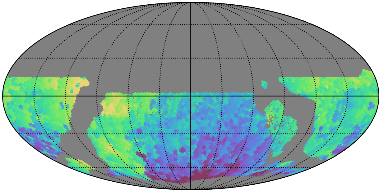
ddf_loaded_half_f14_v3.4_10yrs WFD y band: Min HA
