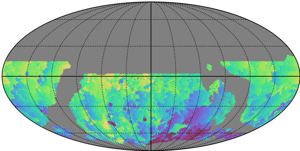
ddf_loaded_half_fl4_v3.4_10yrs WFD u band: Min HA
