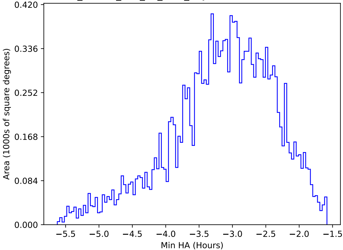
ddf_loaded_half_fl4_v3.4_10yrs WFD u band: Min HA
