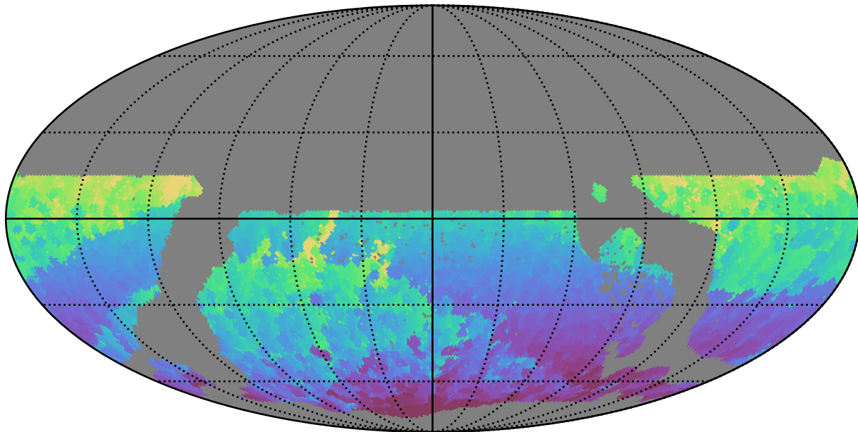
ddf_loaded_half_fl4_v3.4_10yrs WFD r band: Min HA
