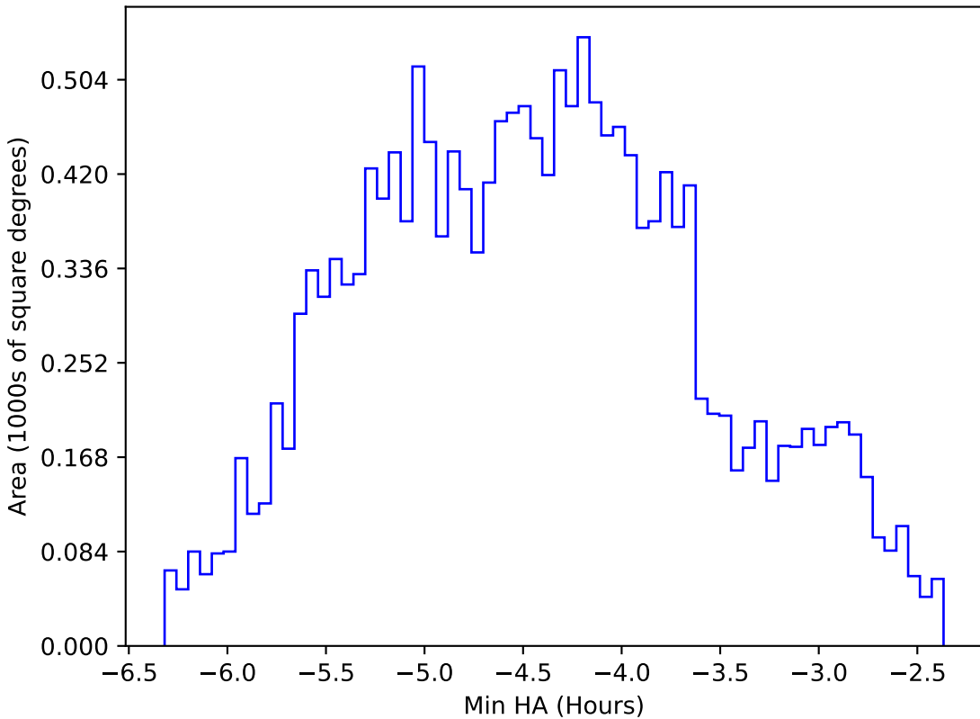
ddf_loaded_half_fl4_v3.4_10yrs WFD r band: Min HA
