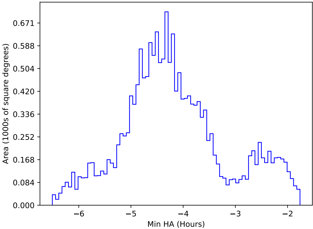
ddf_loaded_half_fl4_v3.4_10yrs WFD g band: Min HA
