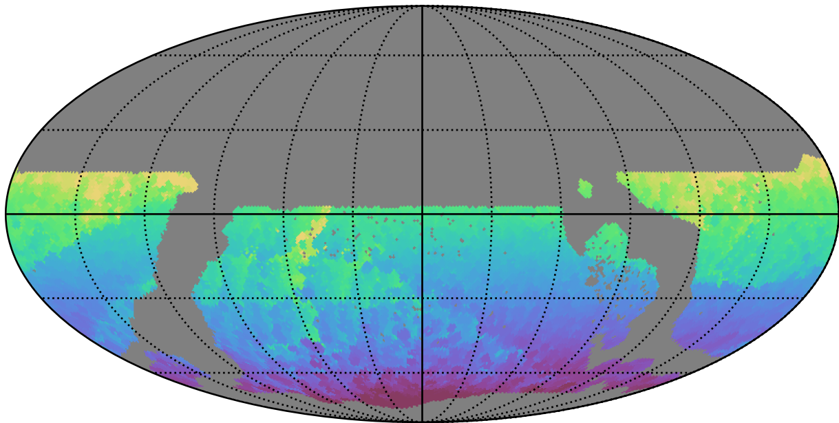
ddf_loaded_half_fl4_v3.4_10yrs WFD all bands: Min HA
