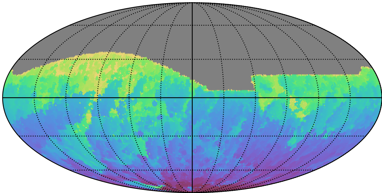
ddf_loaded_half_fl4_v3.4_10yrs All sky z band: Min HA
