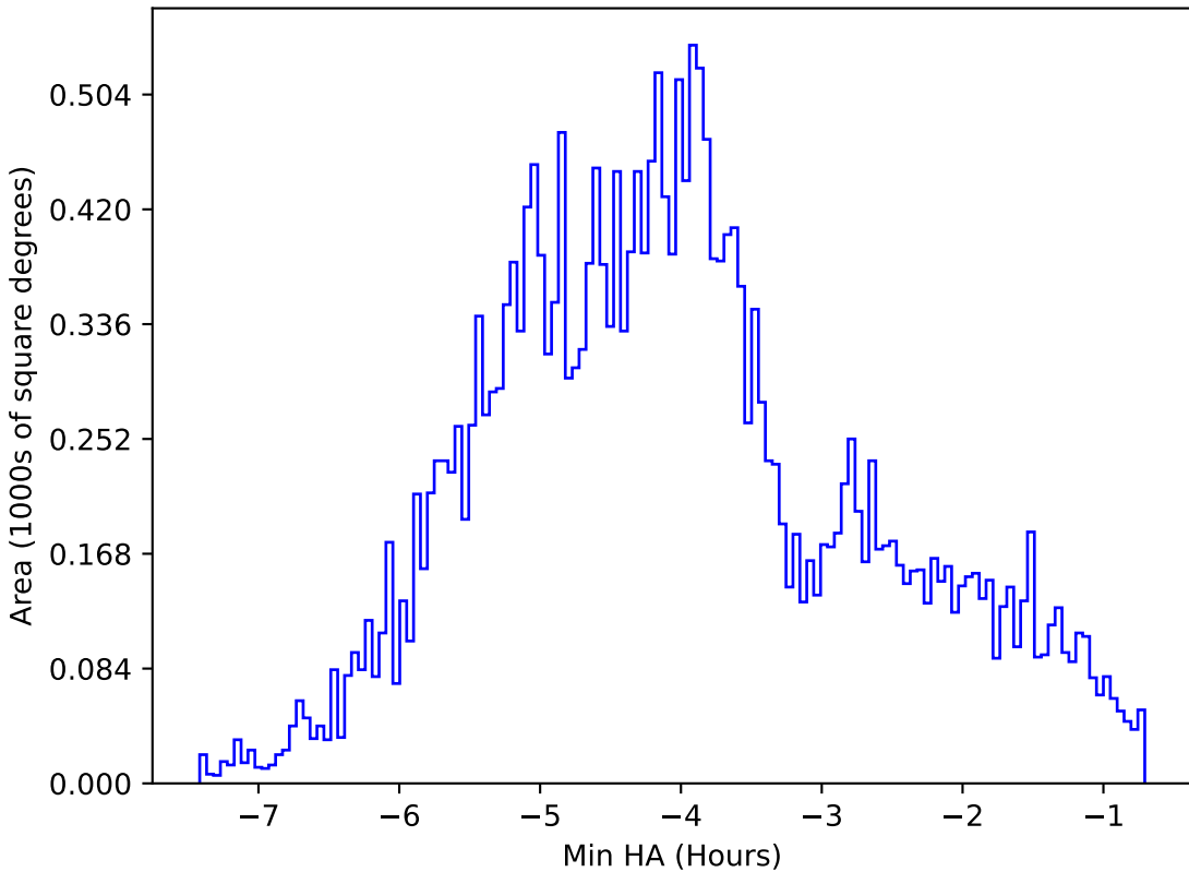
ddf_loaded_half_fl4_v3.4_10yrs All sky z band: Min HA
