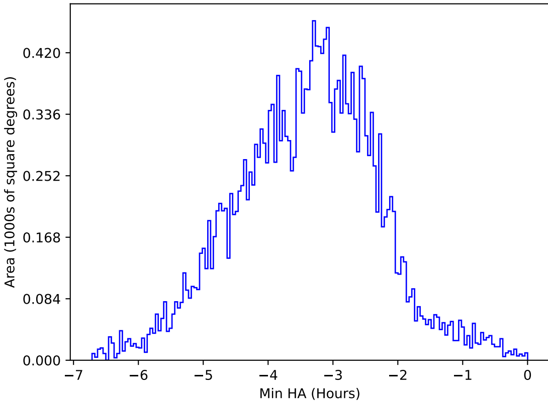
ddf_loaded_half_fl4_v3.4_10yrs All sky y band: Min HA
