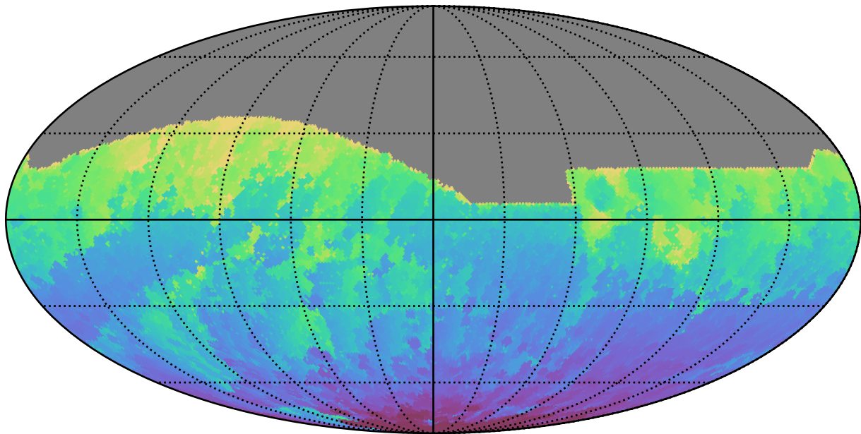
ddf_loaded_half_fl4_v3.4_10yrs All sky i band: Min HA
