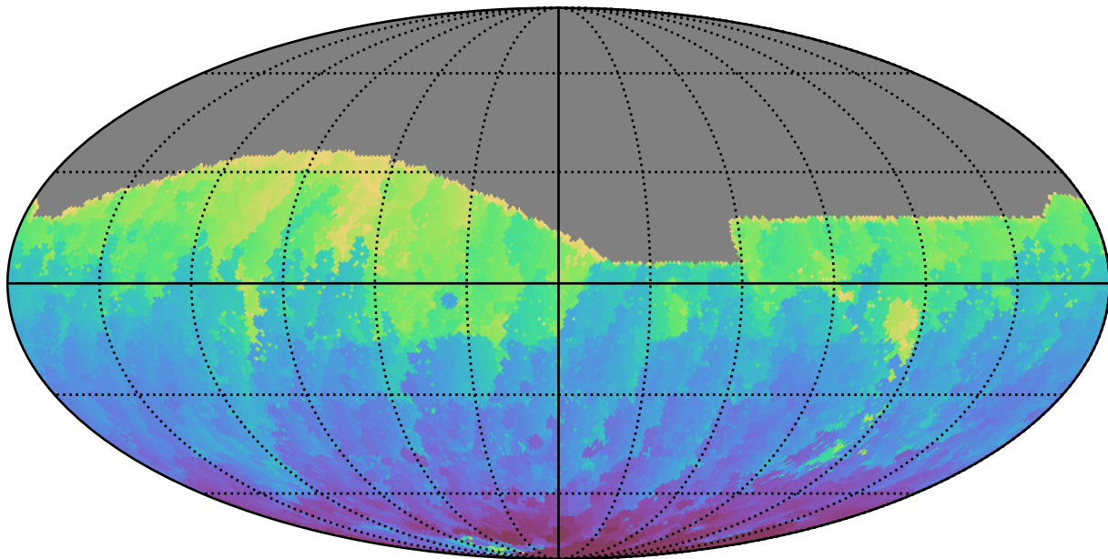
ddf_loaded_half_f14_v3.4_10yrs All sky g band: Min HA
