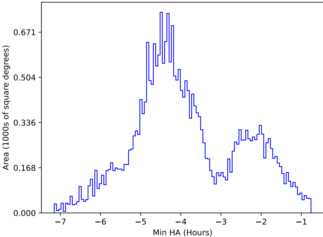
ddf_loaded_half_fl4_v3.4_10yrs All sky g band: Min HA
