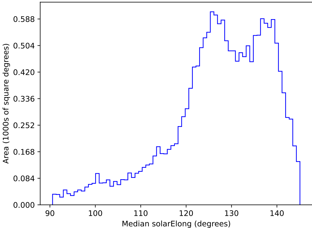
ddf_loaded_half_fl4_v3.4_10yrs WFD z band: Median solarElong
